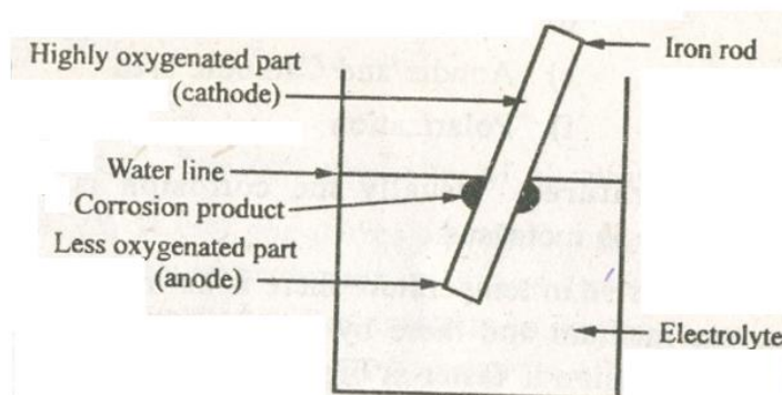
Fig. 2.1: Electrochemical theory of corrosion
